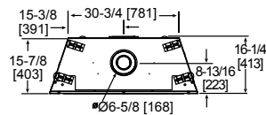
Top View Corner Installation
